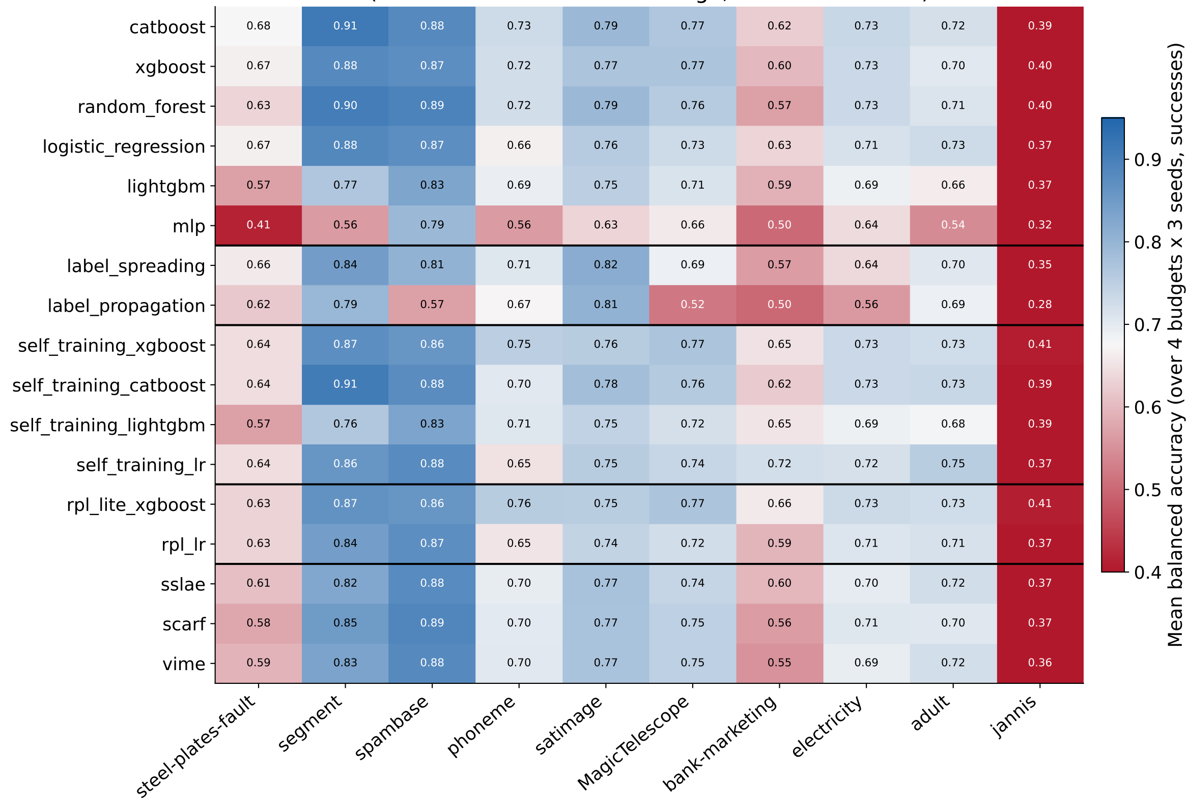
Method x dataset — mean balanced accuracy (datasets ordered small -> large; failures excluded)
