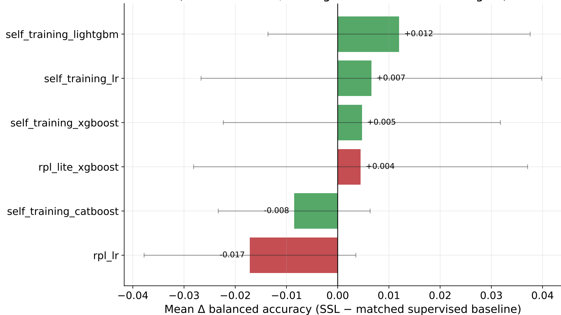
SSL vs matched supervised baseline (matched seeds; averaged over datasets x budgets)
