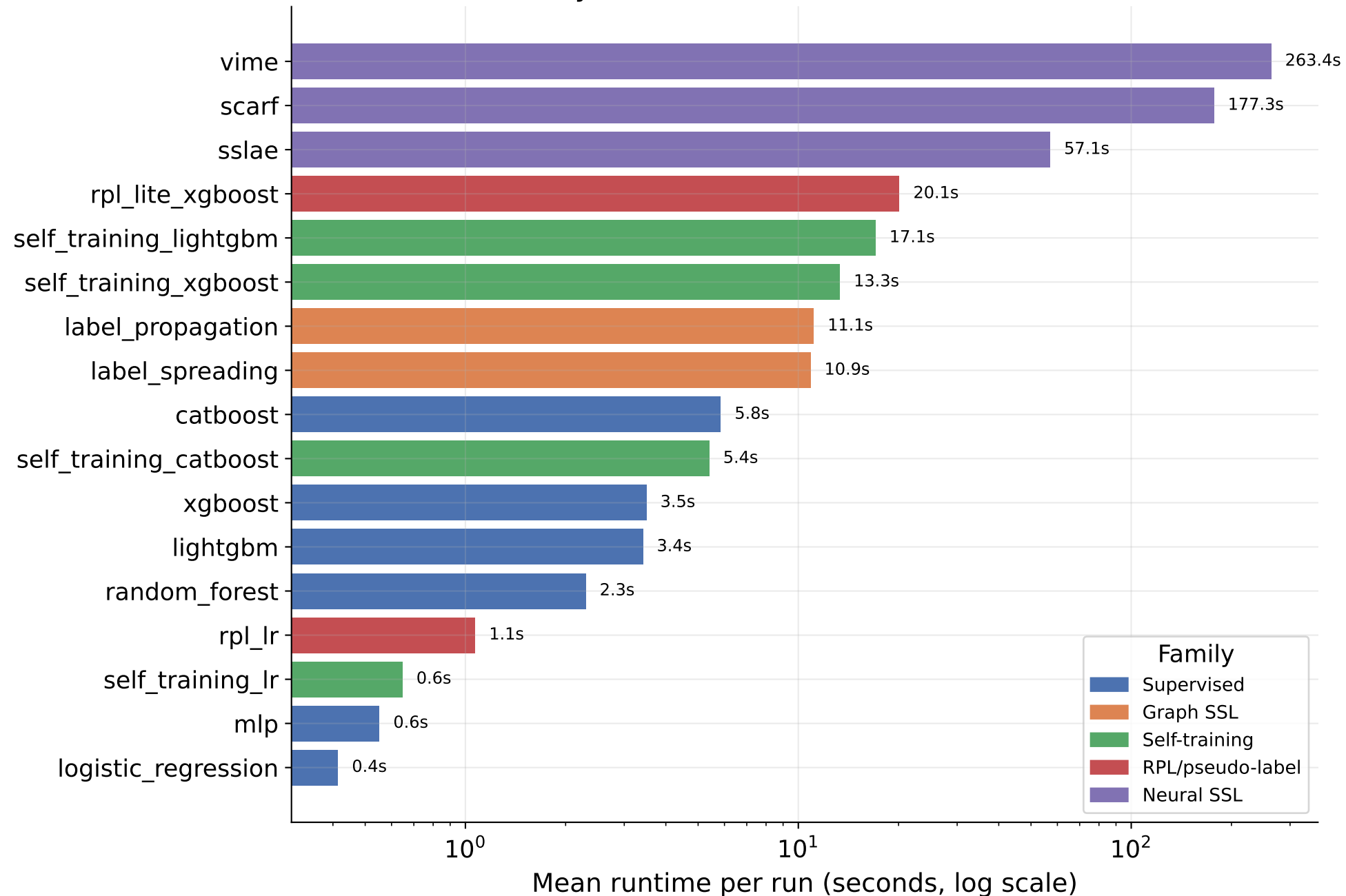
Runtime by method (mean over all successful runs)
