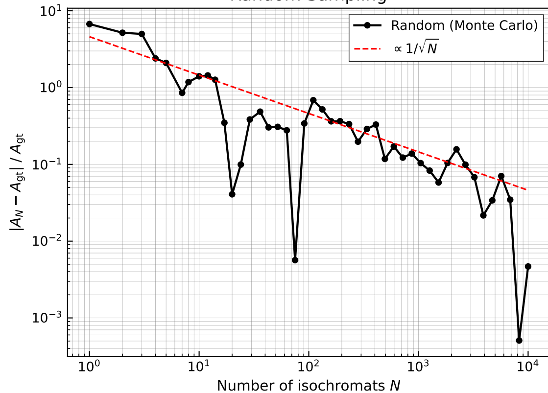
Random Sampling
