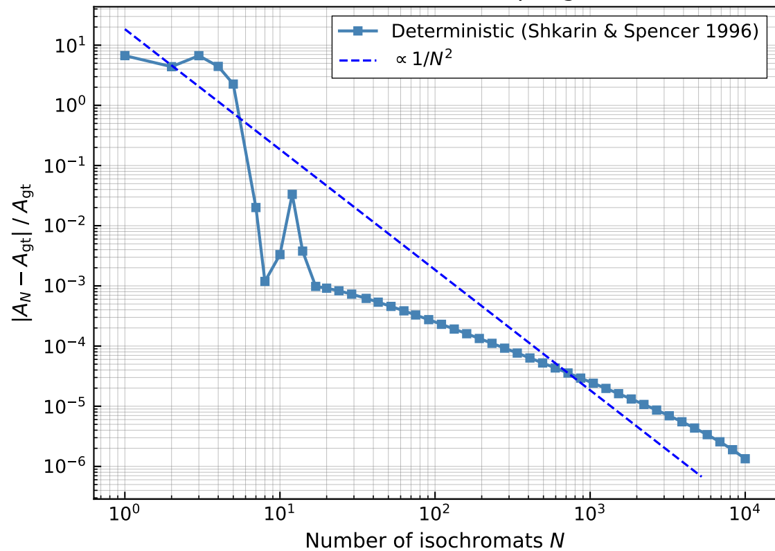
Deterministic Sampling
