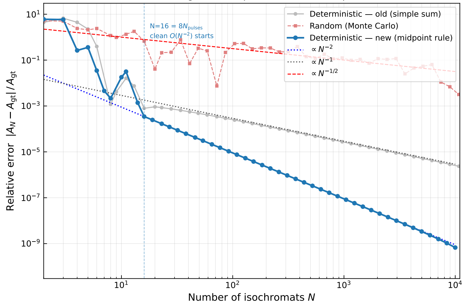
Isochromat convergence: midpoint rule vs. old implementation
