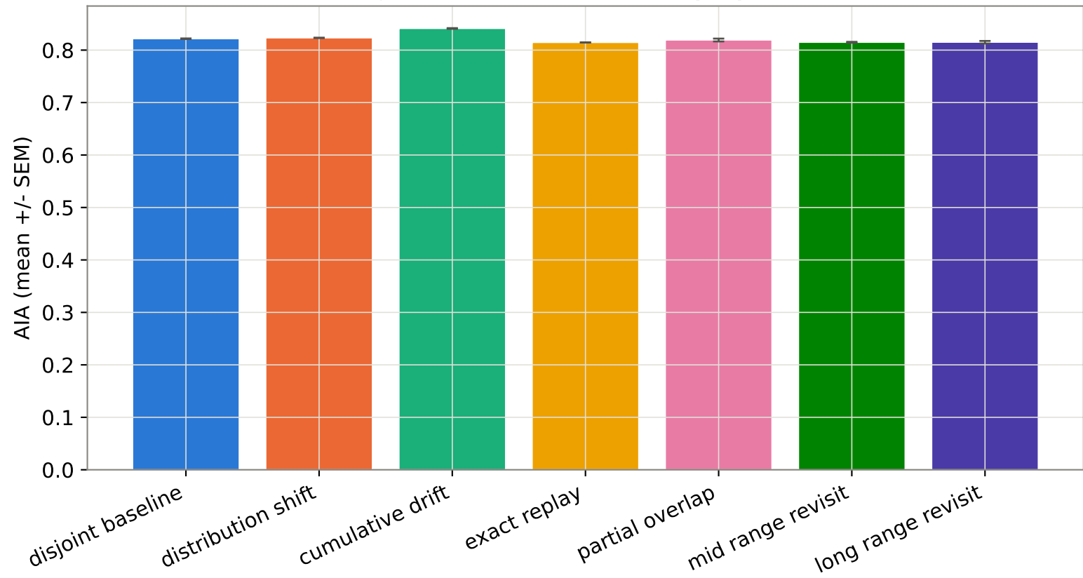
Average incremental accuracy by scenario
