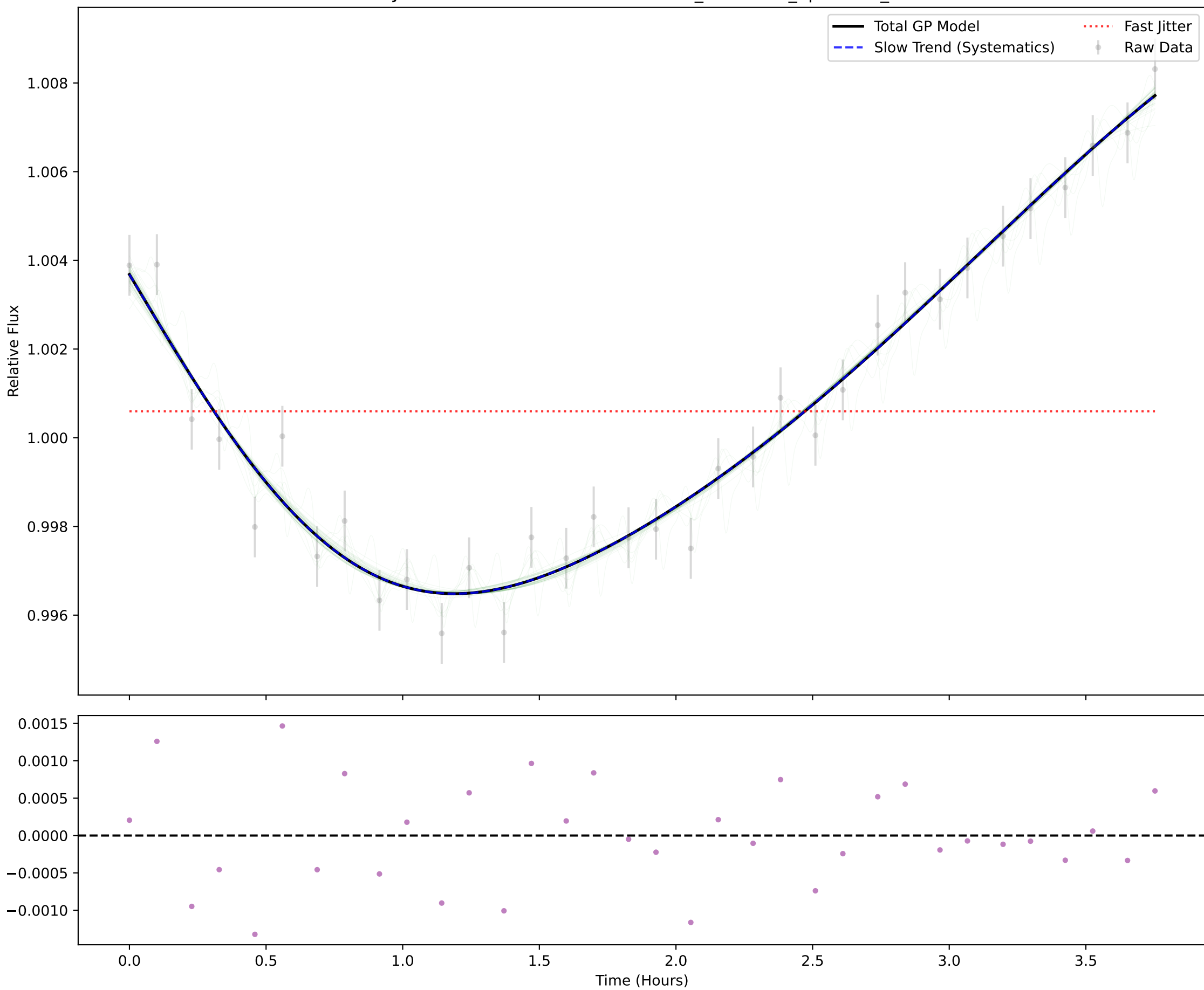
PSO318 Jitter Correction - Visit: 2025-10-01_combined_SpecData_modified
