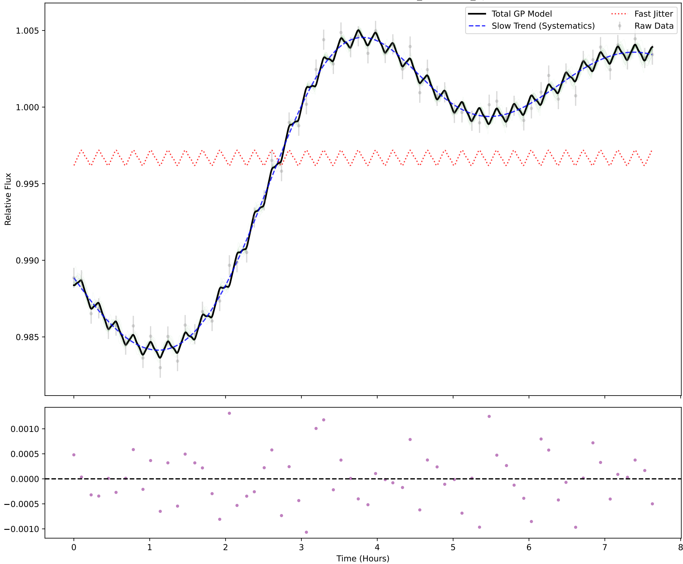
PSO318 Jitter Correction - Visit: 2025-10-21_combined_SpecData
