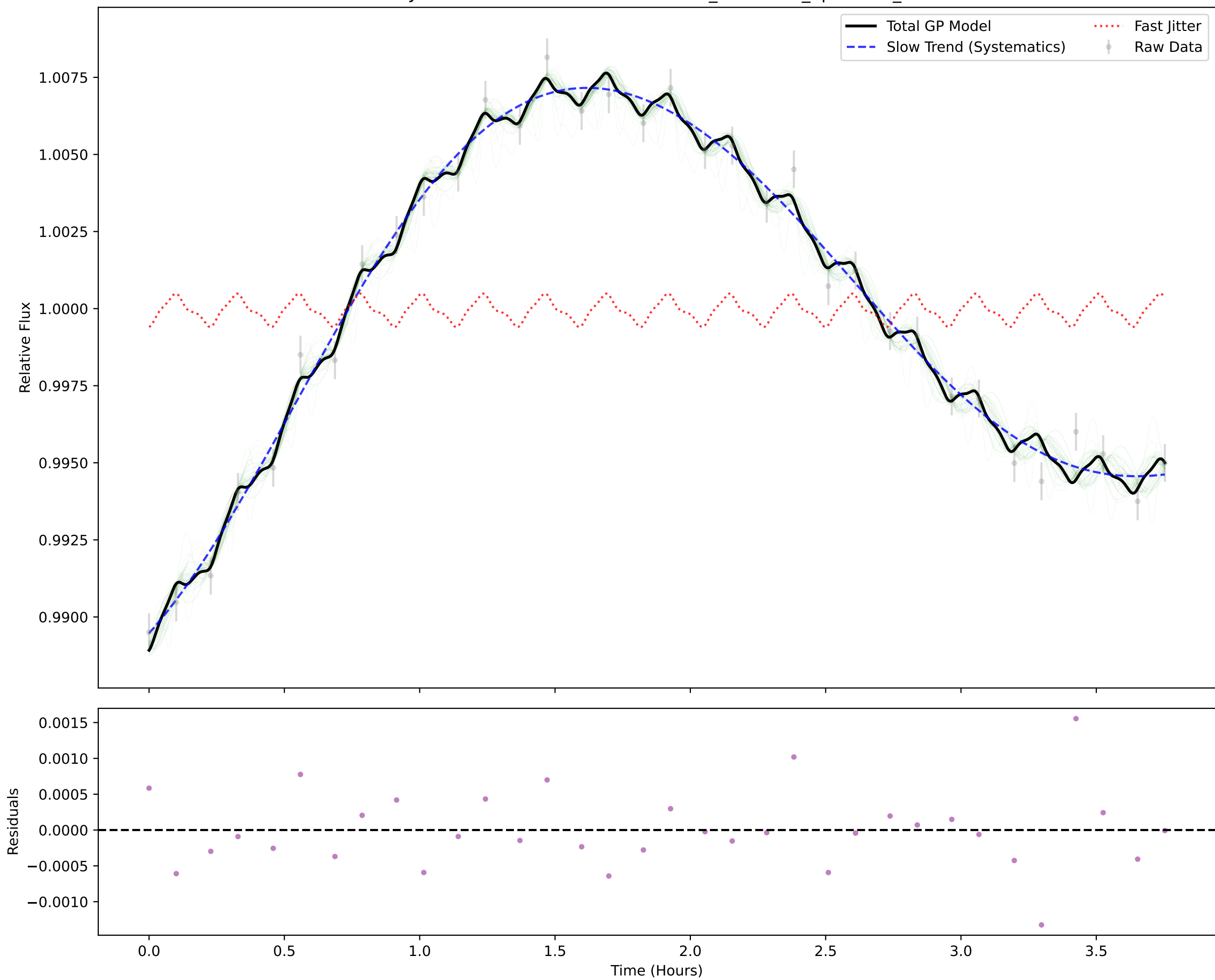
PSO318 Jitter Correction - Visit: 2025-10-21_combined_SpecData_modified
