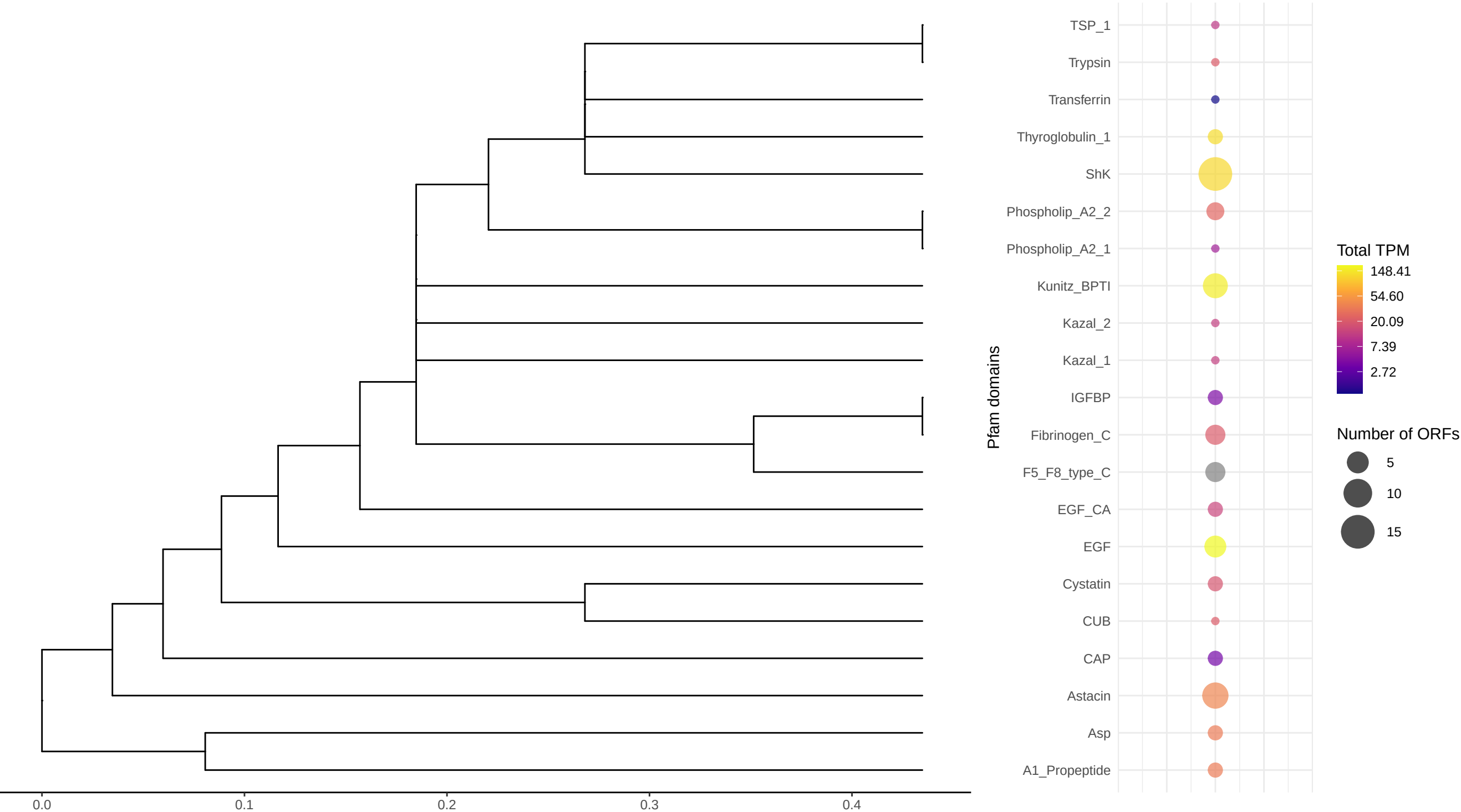
Hierarchical Clustering of Pfam Domains Based on ORF Presence
