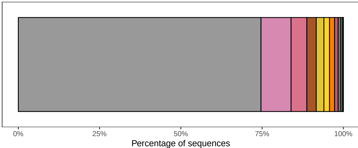
StackedBar_DeTox_Flags_Sorted
