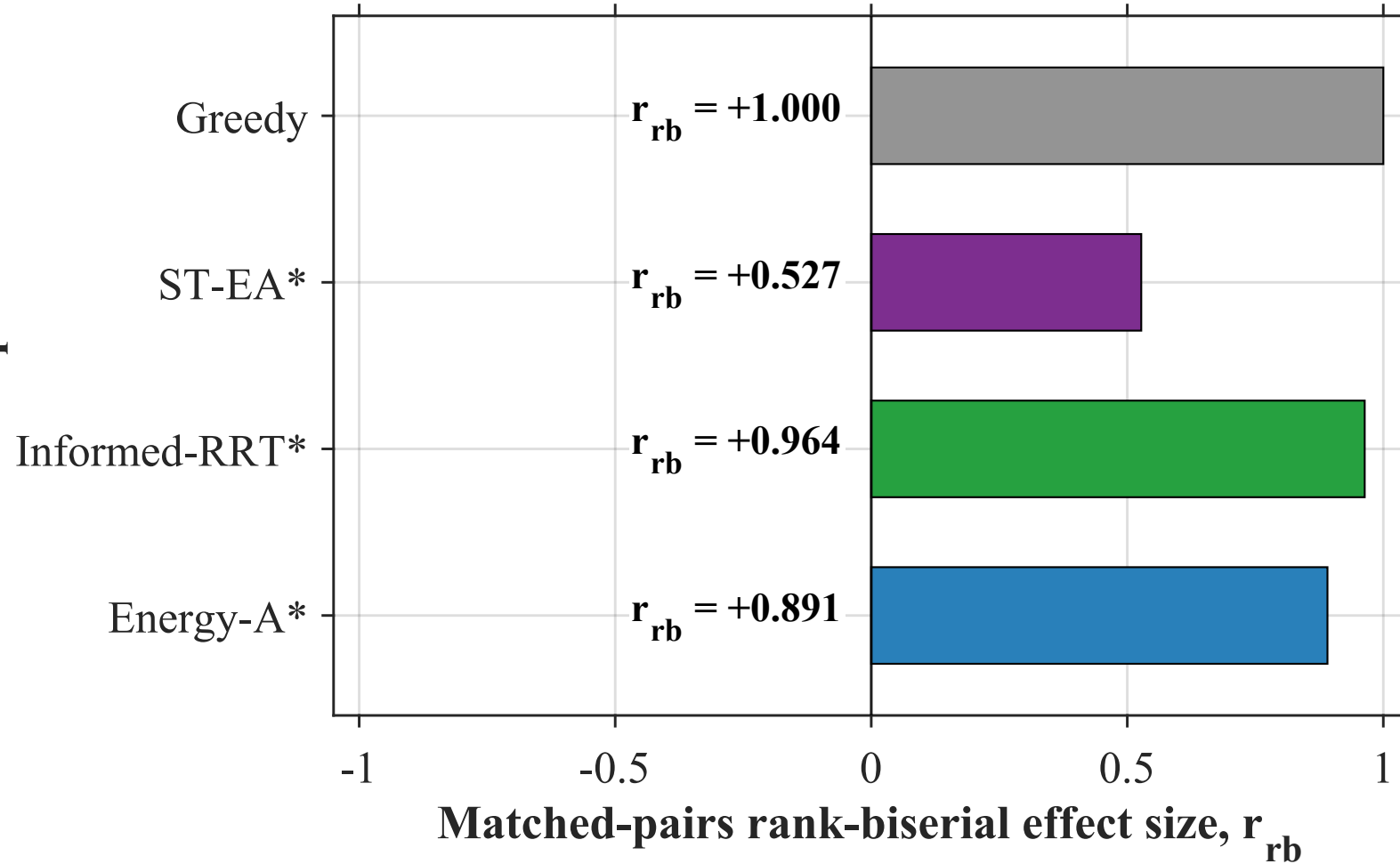
Paired Effect Size: Unified Cost J
