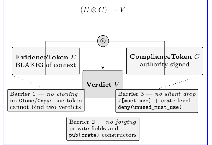
Fig. 3. The core type law (E \otimes C) \multimap V : an EvidenceToken and a ComplianceToken are jointly consumed ( \otimes ) to construct a Verdict ; compiler-enforced barriers block cloning, forging, and silent discarding of tokens.
