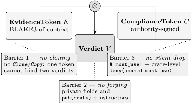
Fig. 3. The core type law (E \otimes C) \multimap V : an EvidenceToken and a ComplianceToken are jointly consumed ( \otimes ) to construct a Verdict; compiler-enforced barriers block cloning and unauthorized construction, and diagnose an ignored token-producing expression at the API boundary.
