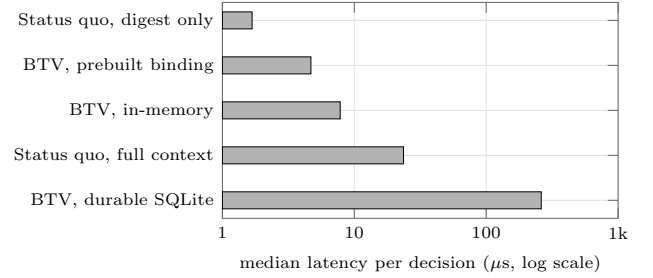
Fig. 5. Measured median latency of the BTV and status-quo logging paths at 4 KiB, one thread (logarithmic scale). The rows compare distinct implementation and persistence postures, not a single end-to-end number; type-level enforcement adds no runtime branch, and the measured costs are those of hashing, token verification, sealing, encoding, and—where enabled—durable persistence.
