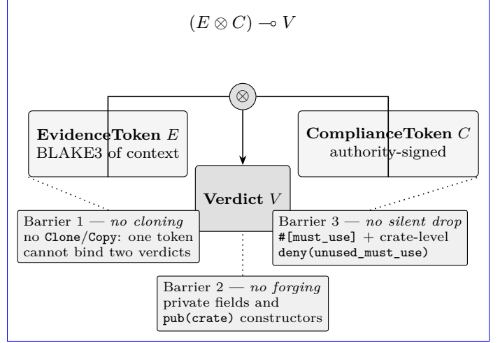
Fig. 3. The core type law (E \otimes C) \multimap V : an EvidenceToken and a ComplianceToken are jointly consumed ( \otimes ) to construct a Verdict; compiler-enforced barriers block cloning and unauthorized construction, and diagnose an ignored token-producing expression at the API boundary.
