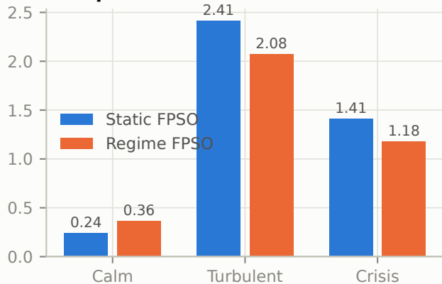
Sharpe ratio
