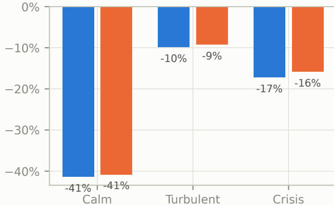
Maximum drawdown
