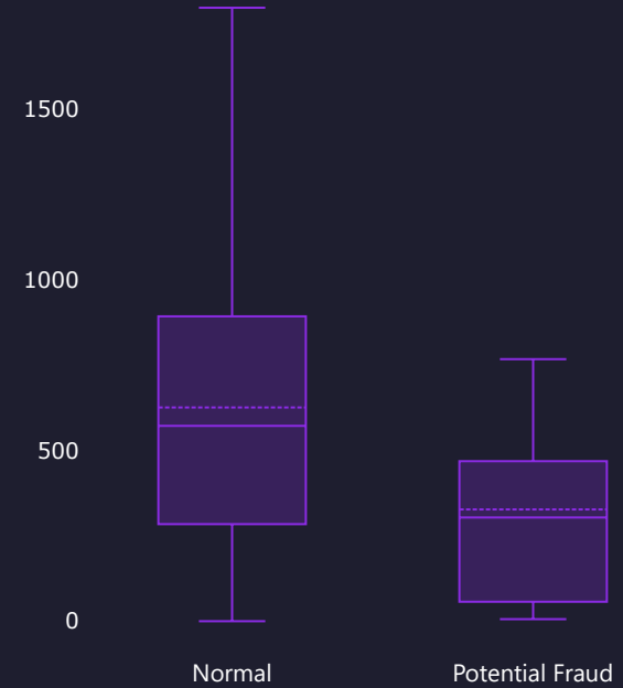
Trans Amount Distribution by Anomaly Label
