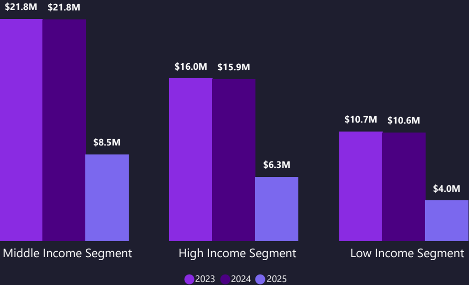
Segment Performance
