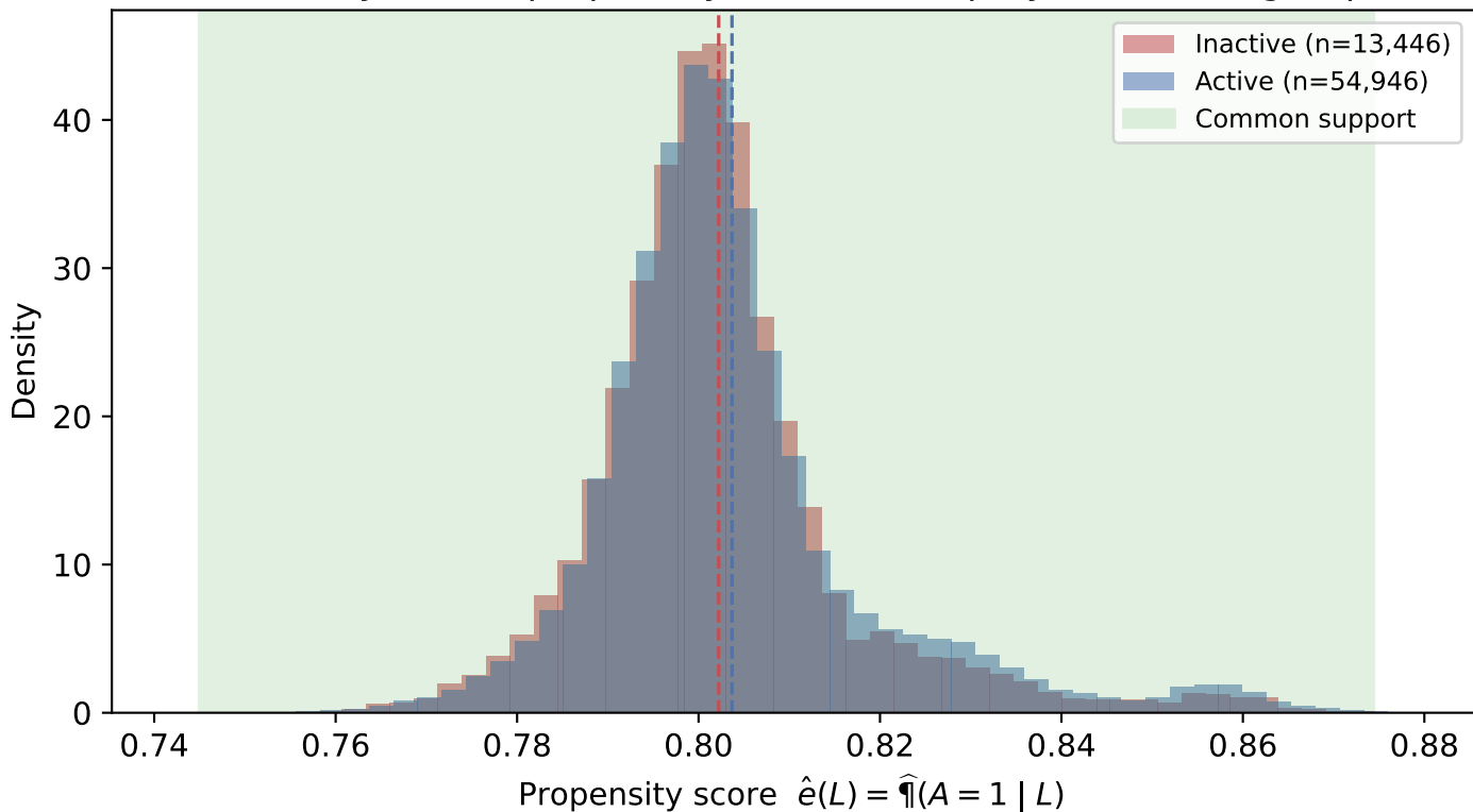
Positivity check: propensity score overlap by treatment group
