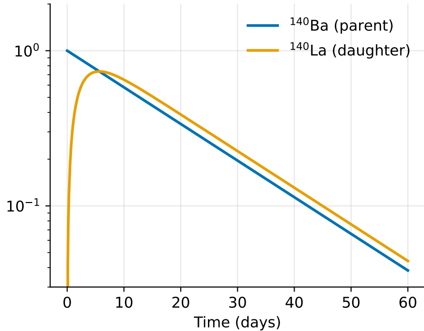
(b) Transient equilibrium
