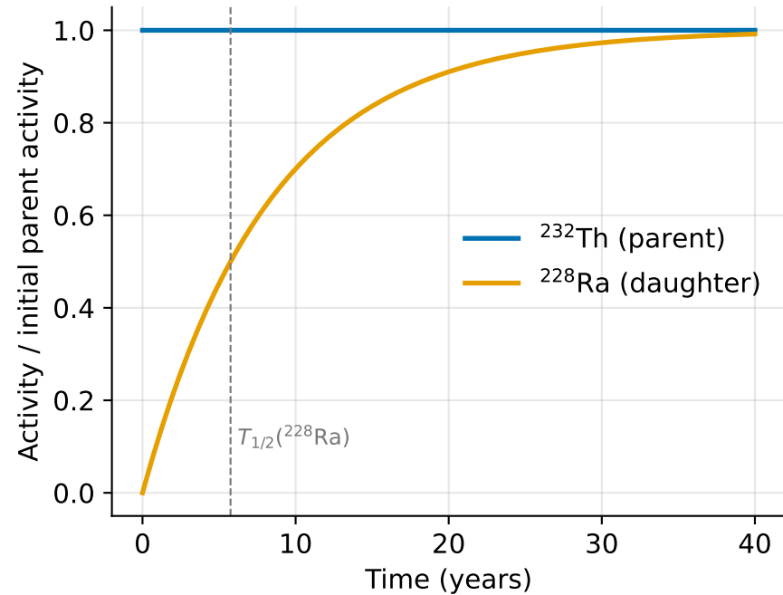
(a) Secular equilibrium
