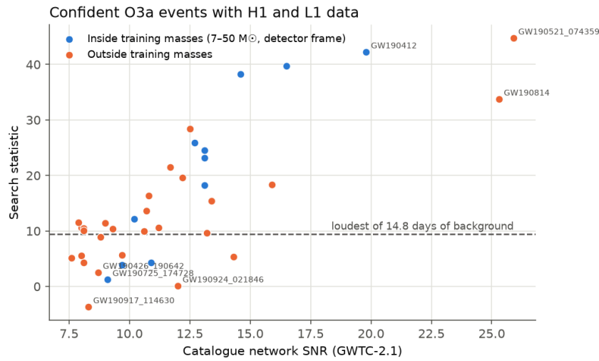
Figure 7. Search statistic of the analysed O3a events against catalogue network SNR. The dashed line marks the loudest background event in 14.8 days.
