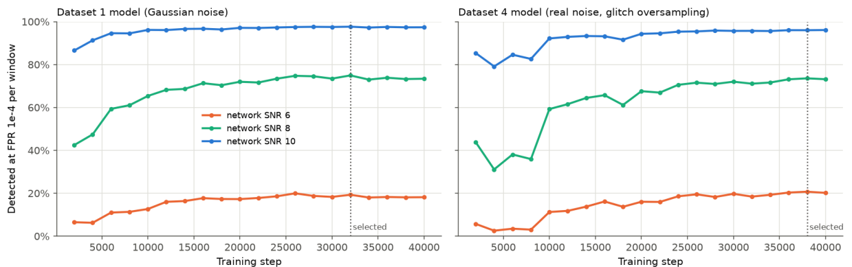
Figure 4. Validation detection fraction at a false-positive probability of 10^{-4} per window, on held-out noise and signals. The dotted line marks the retained checkpoint.
