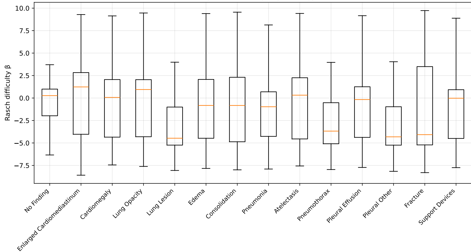
Item difficulty distribution per pathology (Rasch)
