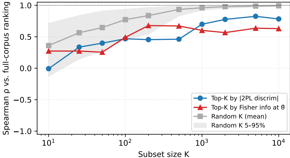
Tiny-benchmark recovery (12 subjects)
