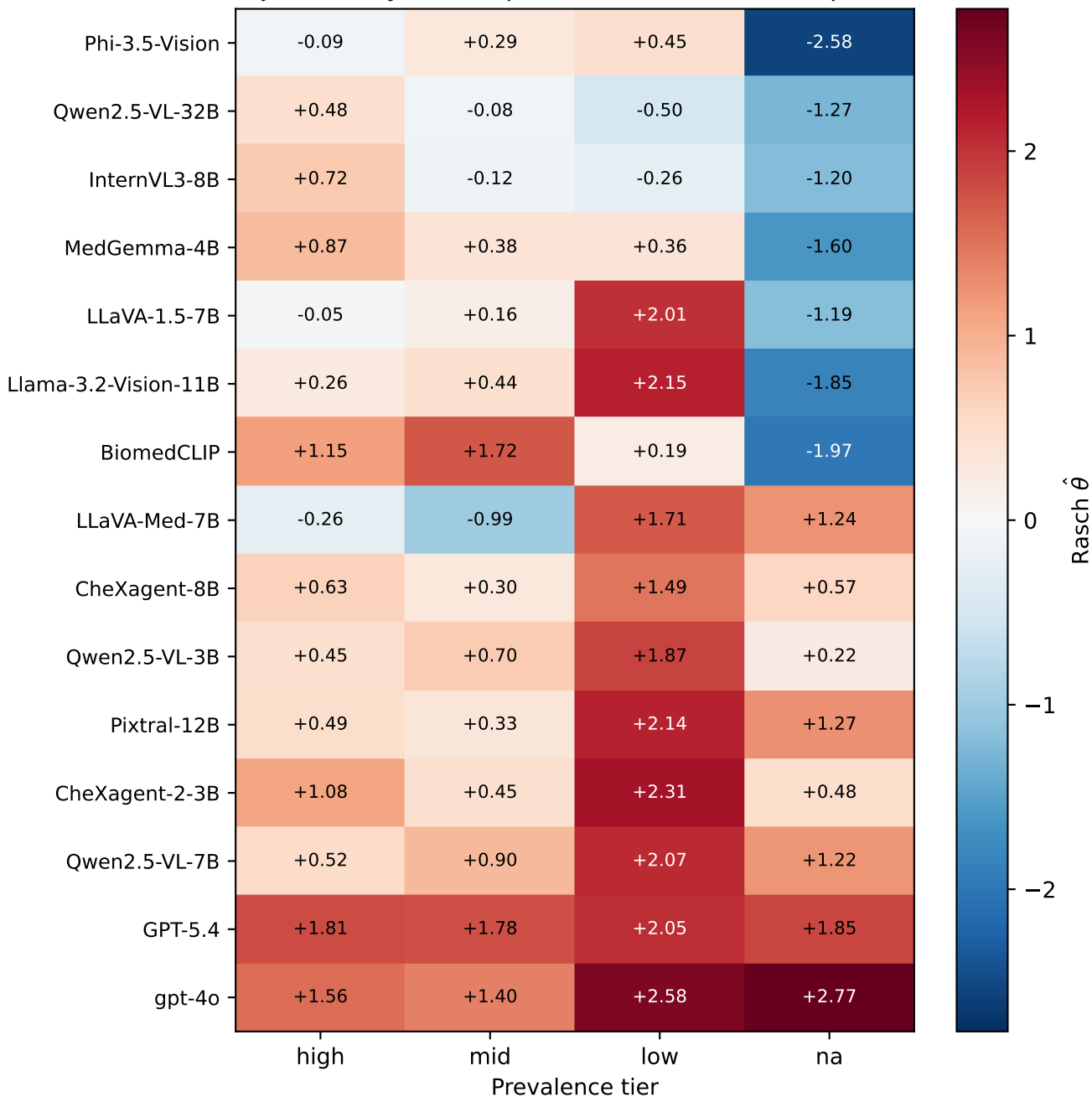
Subject ability across prevalence tiers (Rasch per tier)
