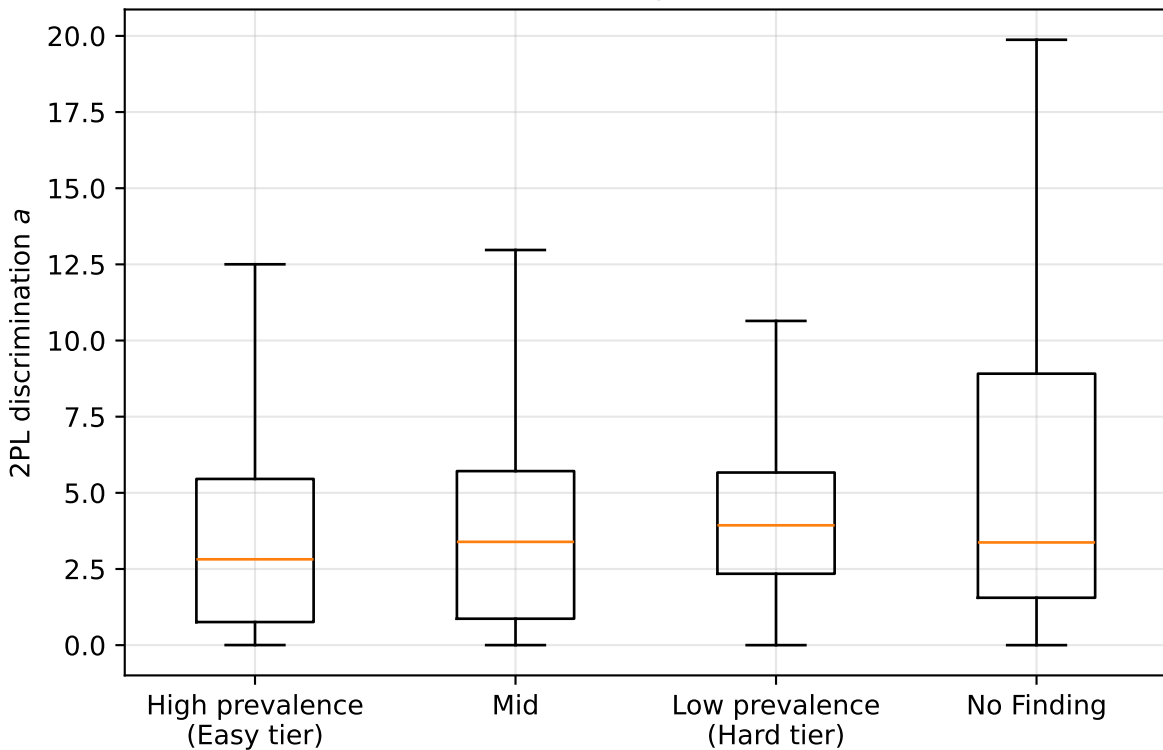
2PL discrimination per prevalence tier (stratified item-pool variation)
