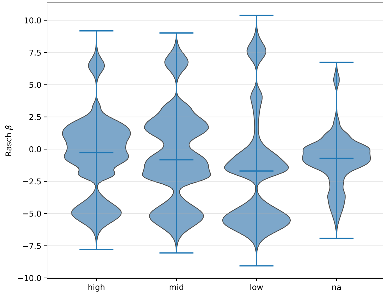
Item difficulty per tier
