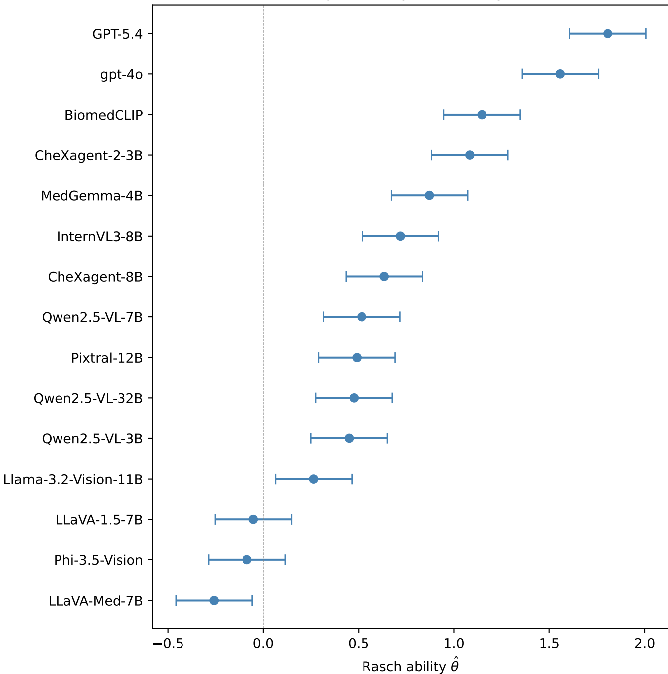
Per-subject ability (Rasch, high tier)
