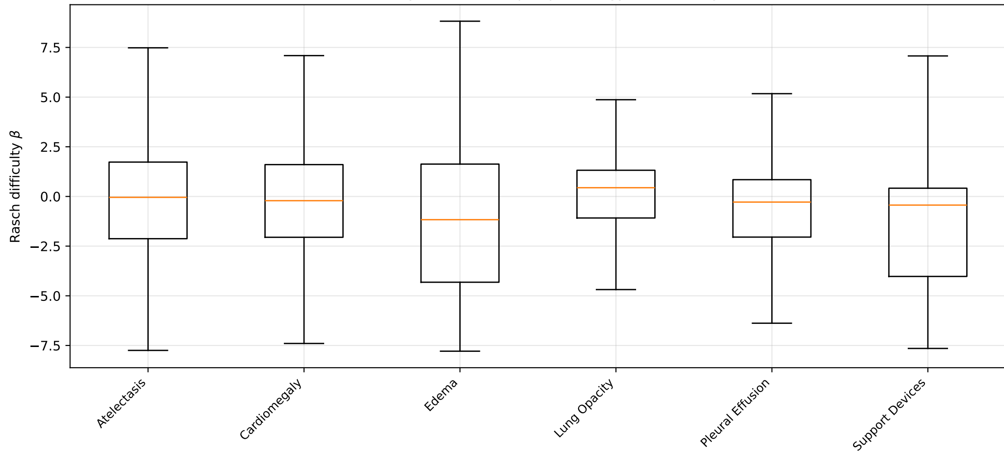
Item difficulty distribution per pathology (Rasch, high tier)
