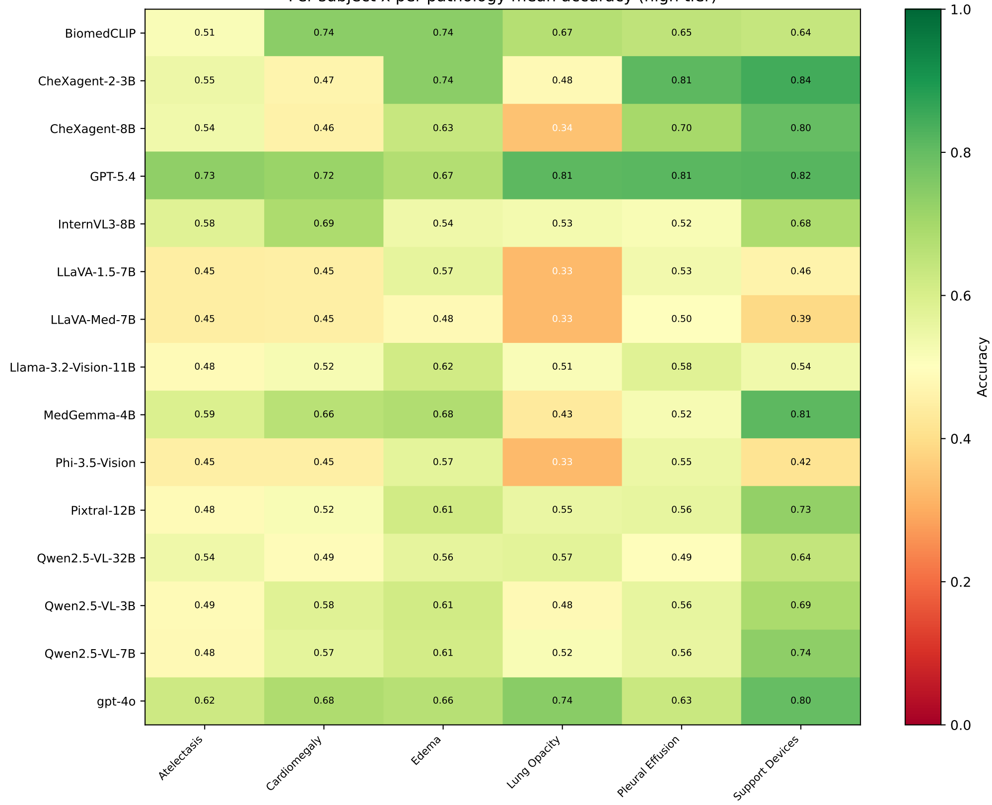
Per-subject x per-pathology mean accuracy (high tier)
