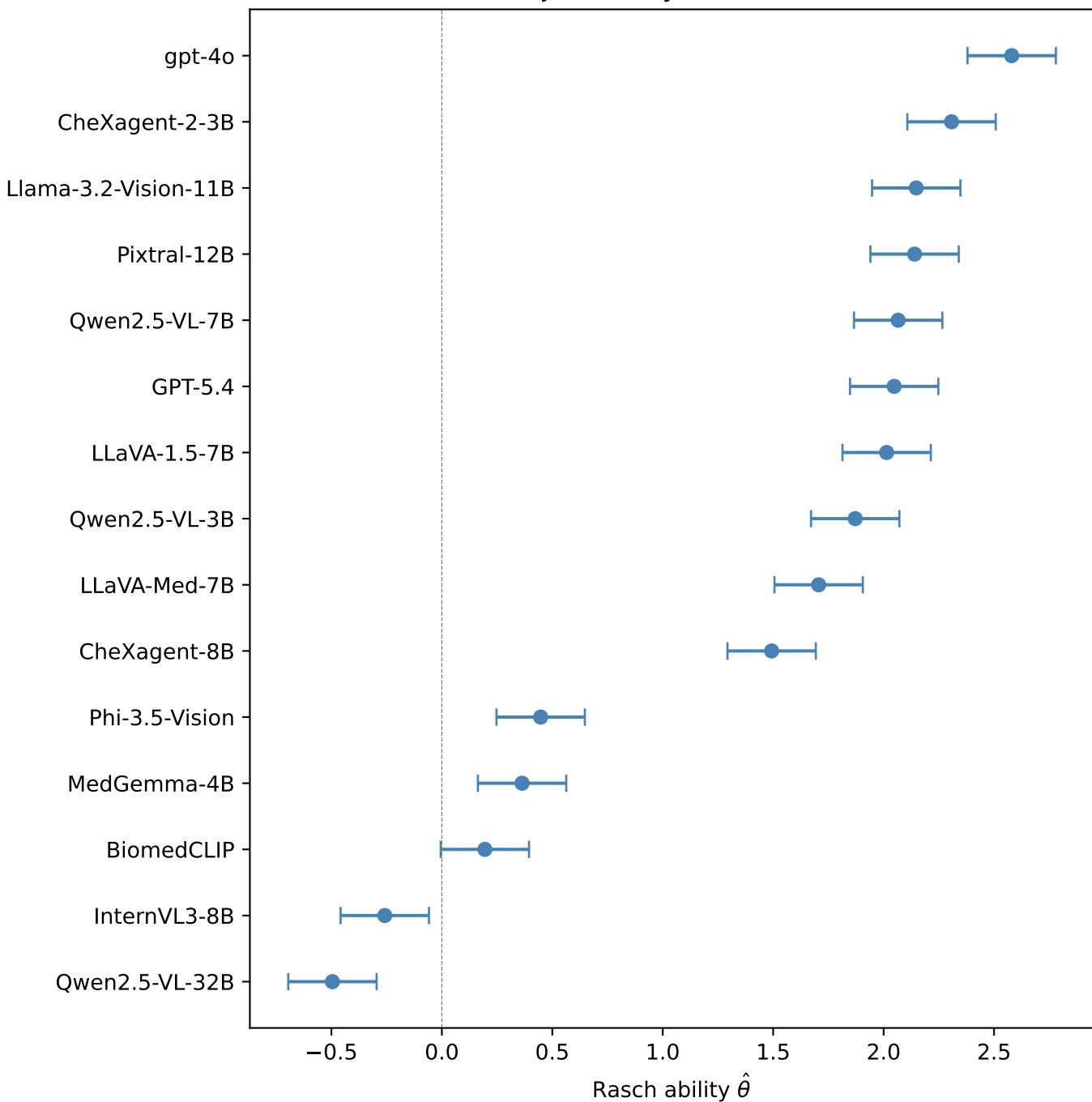
Per-subject ability (Rasch, low tier)
