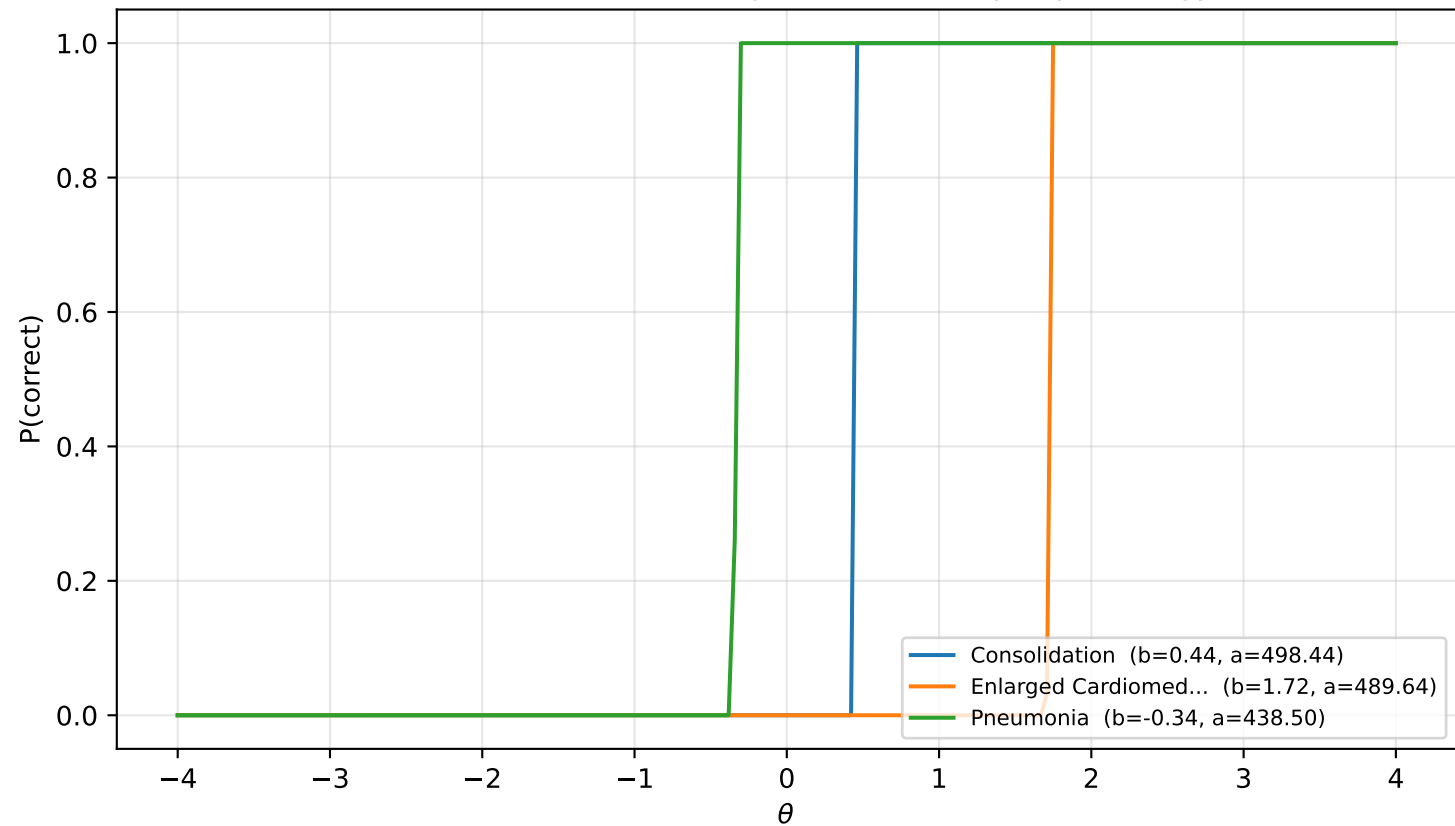
Item characteristic curves (2PL, top-discrim item per pathology, mid tier)
