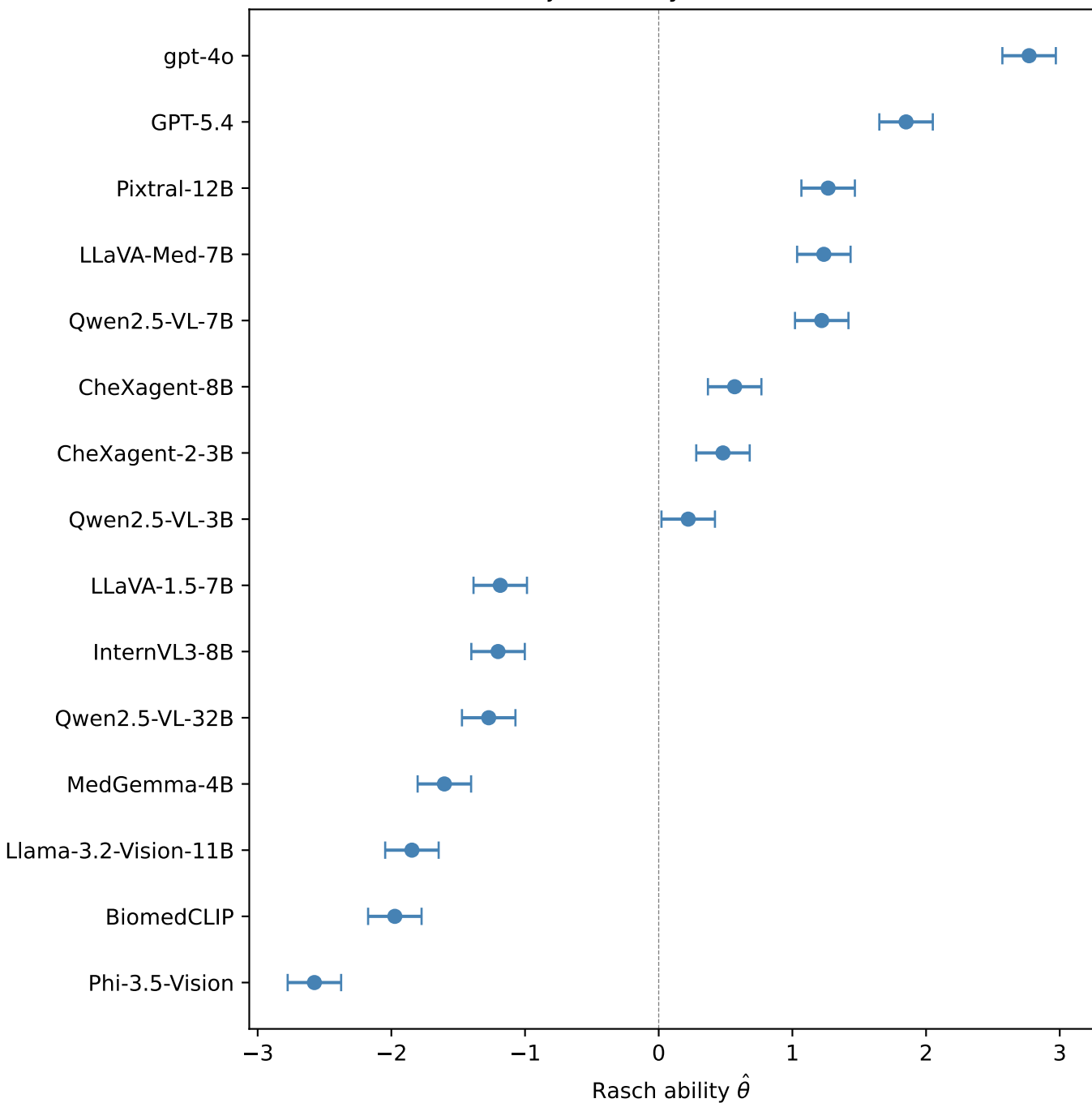
Per-subject ability (Rasch, na tier)
