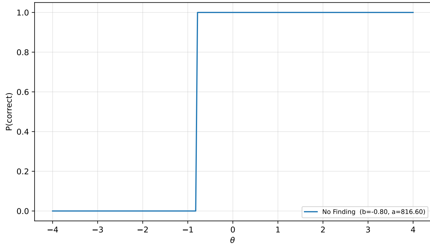
Item characteristic curves (2PL, top-discrimination item per pathology, no tier)
