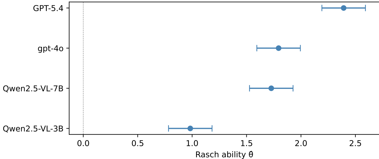
Per-subject ability (Rasch)
