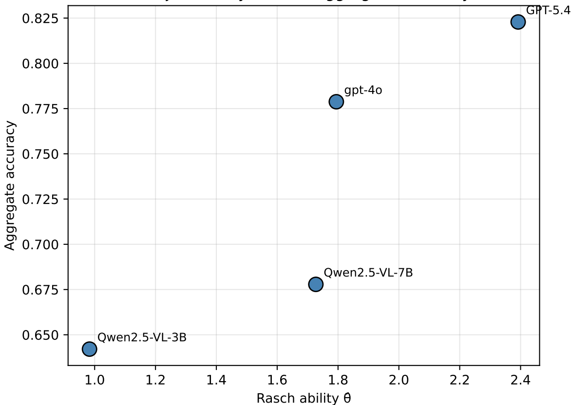
Subject ability (IRT) vs aggregate accuracy
