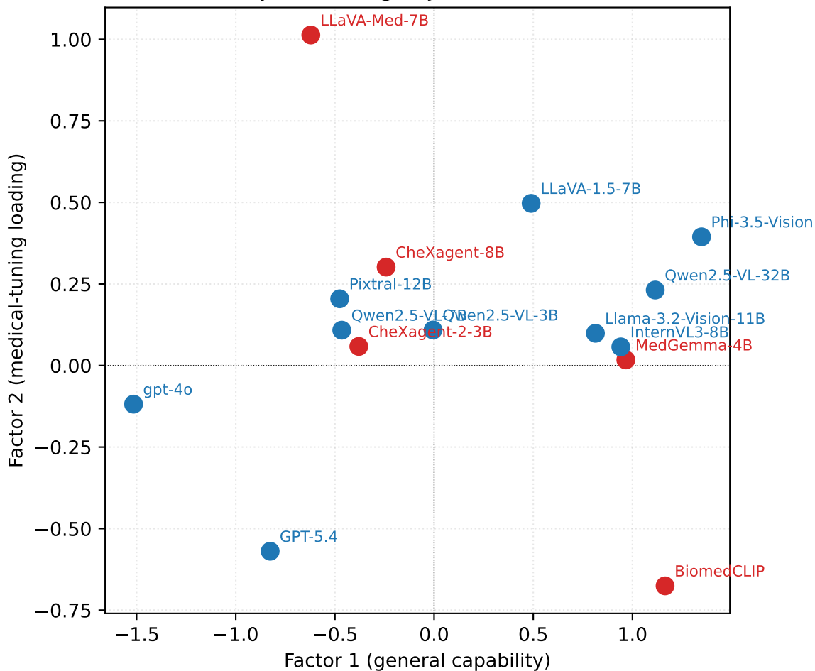
2-D MIRT subject loadings ( J = 15 ) -2\Delta LL = 35066.5
