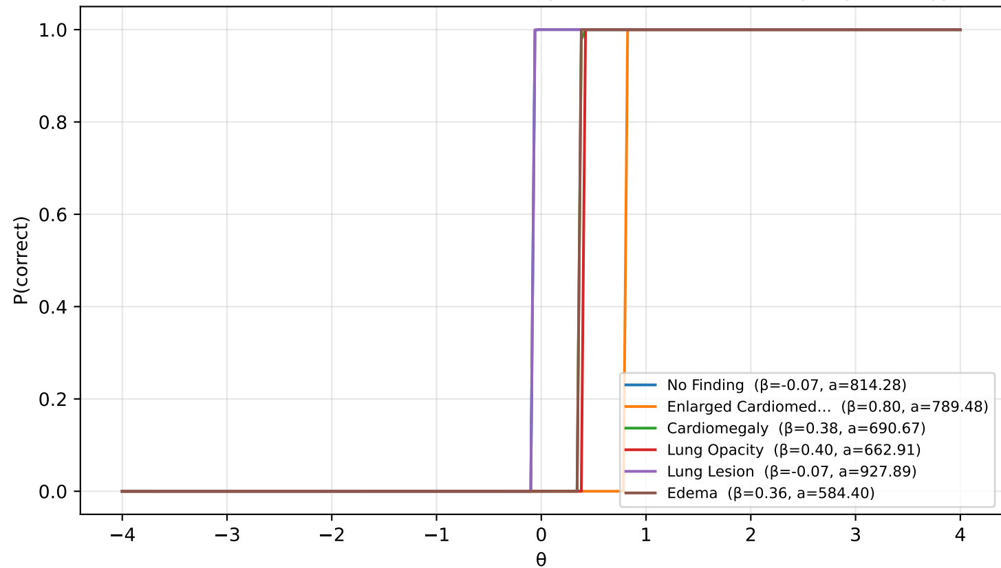
Item characteristic curves (2PL, one high-discrimination item per pathology)
