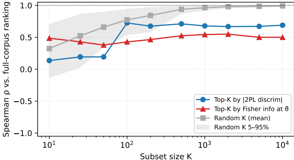
Tiny-benchmark recovery (15 subjects)
