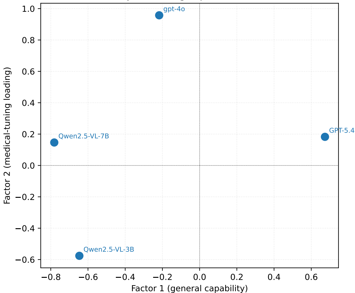
2-D MIRT subject loadings ( J = 4 ) -2\Delta LL = 1668.7
