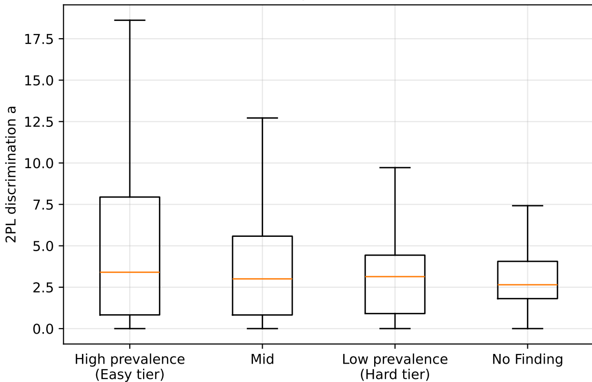
Discrimination spread within prevalence tier (stratification cannot capture this within-tier variation)
