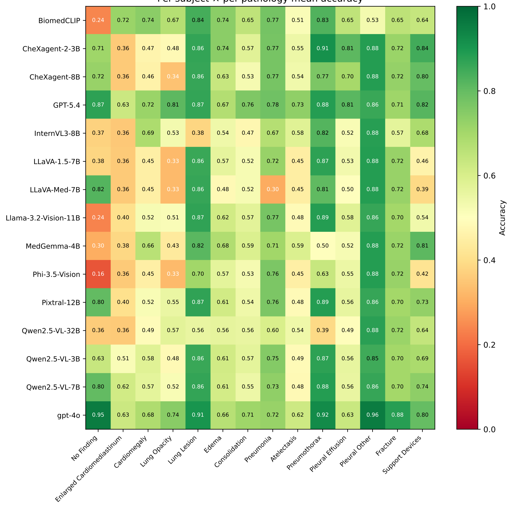
Per-subject × per-pathology mean accuracy
