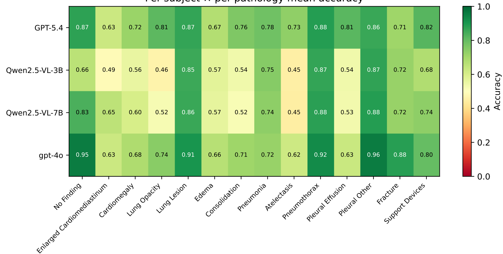
Per-subject × per-pathology mean accuracy
