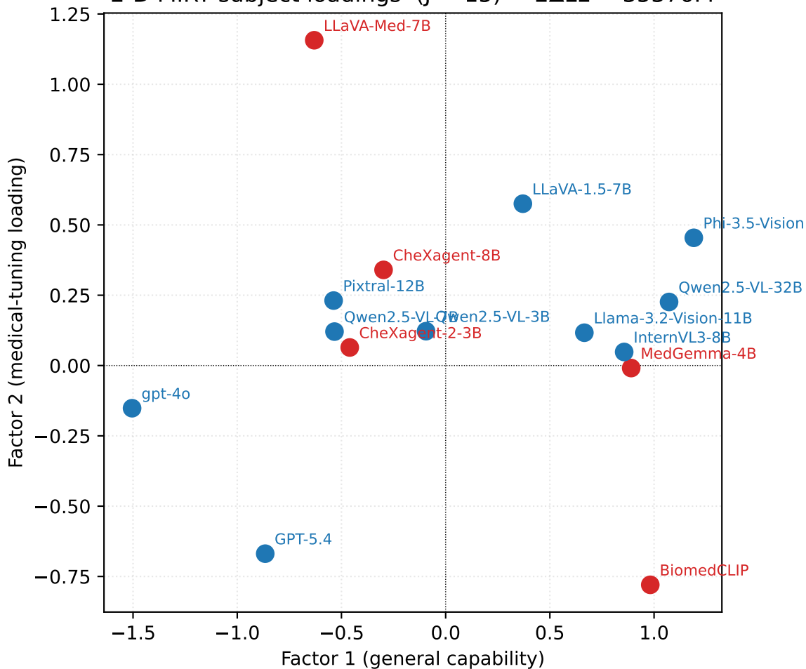
2-D MIRT subject loadings ( J = 15 ) -2\Delta LL = 35376.4
