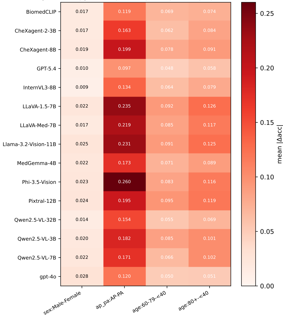
Mean |\Delta\text{accuracy}| across pathologies, by demographic comparison
