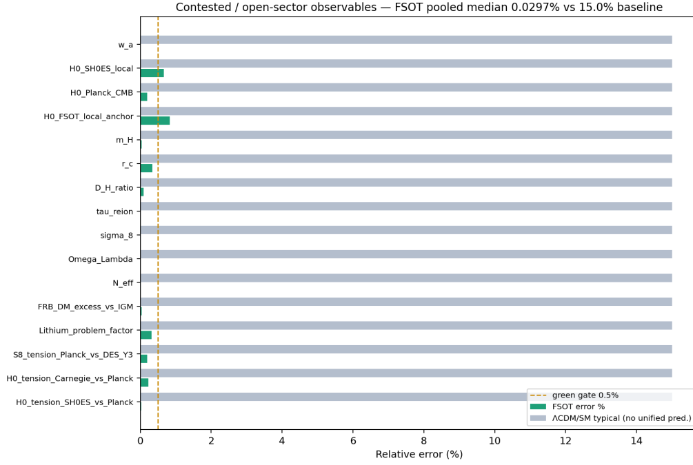
Figure 2: Contested-sector FSOT errors versus typical open-panel baseline scale. Artifact: data/figures/contested_fsot_vs_lcdmd.png . Regenerate with python scripts/build_scientific_figures.py or the publication verification bundle.
