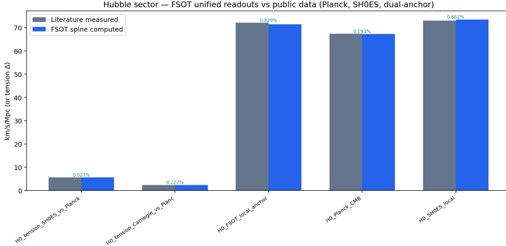
Figure 1: H_0 landscape: dual-anchor routes and FSOT bridge. Artifact: data/figures/h0_landscape.png . One-line regenerate (from a clone of [5]): python scripts/build_scientific_figures.py (also produced by python scripts/run_publication_verification_bundle.py ).
