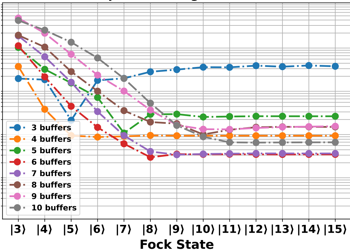
20 blocks (penalize largest 3 fock states)
