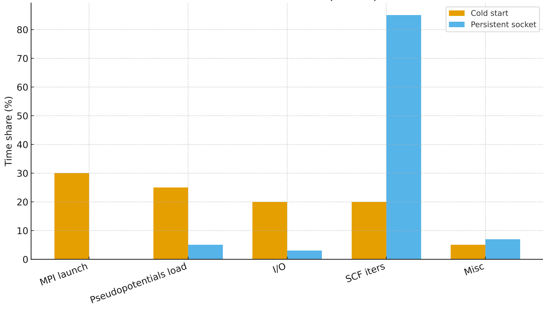
Overhead breakdown per step
