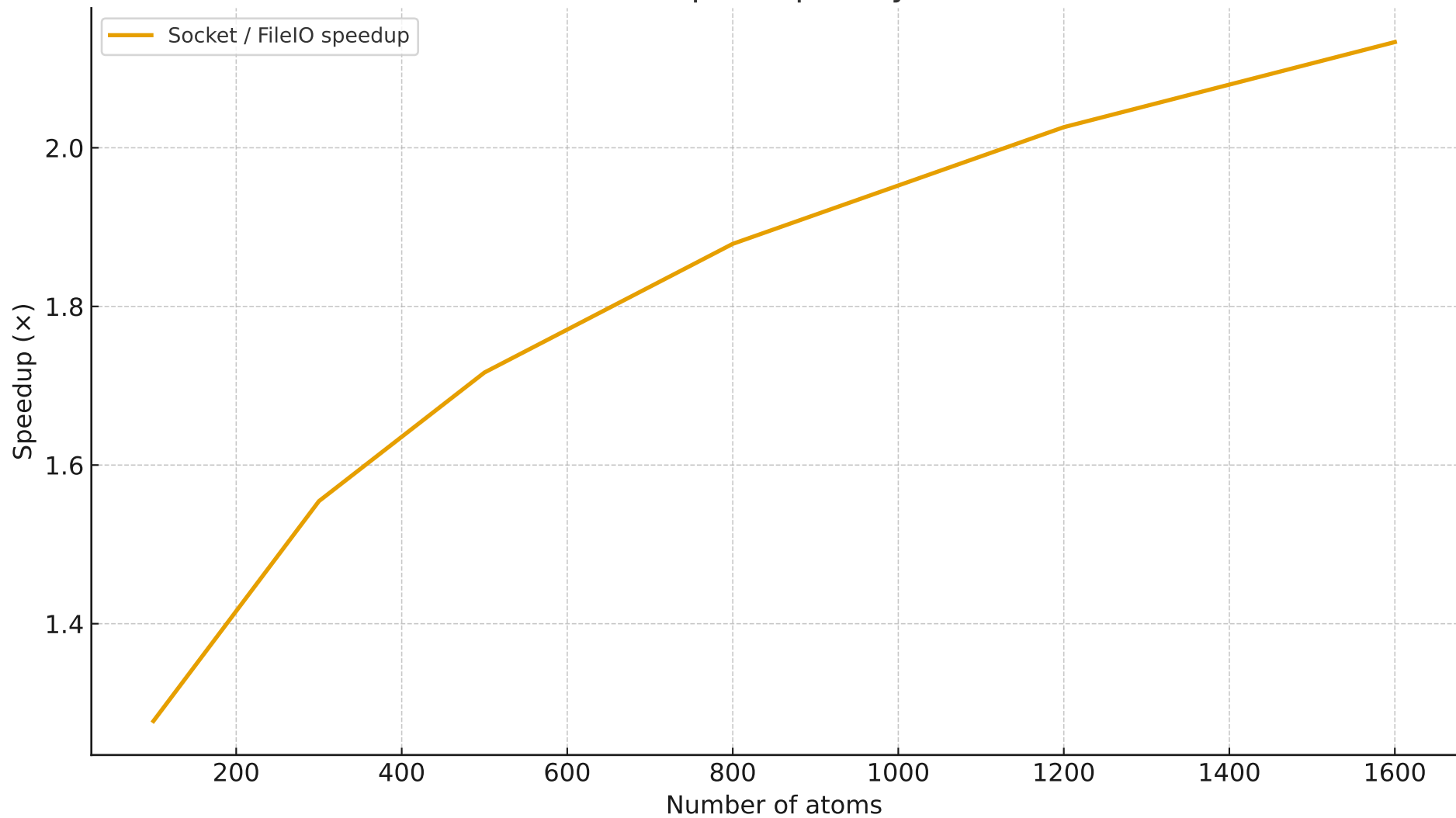
End-to-end speedup vs system size
