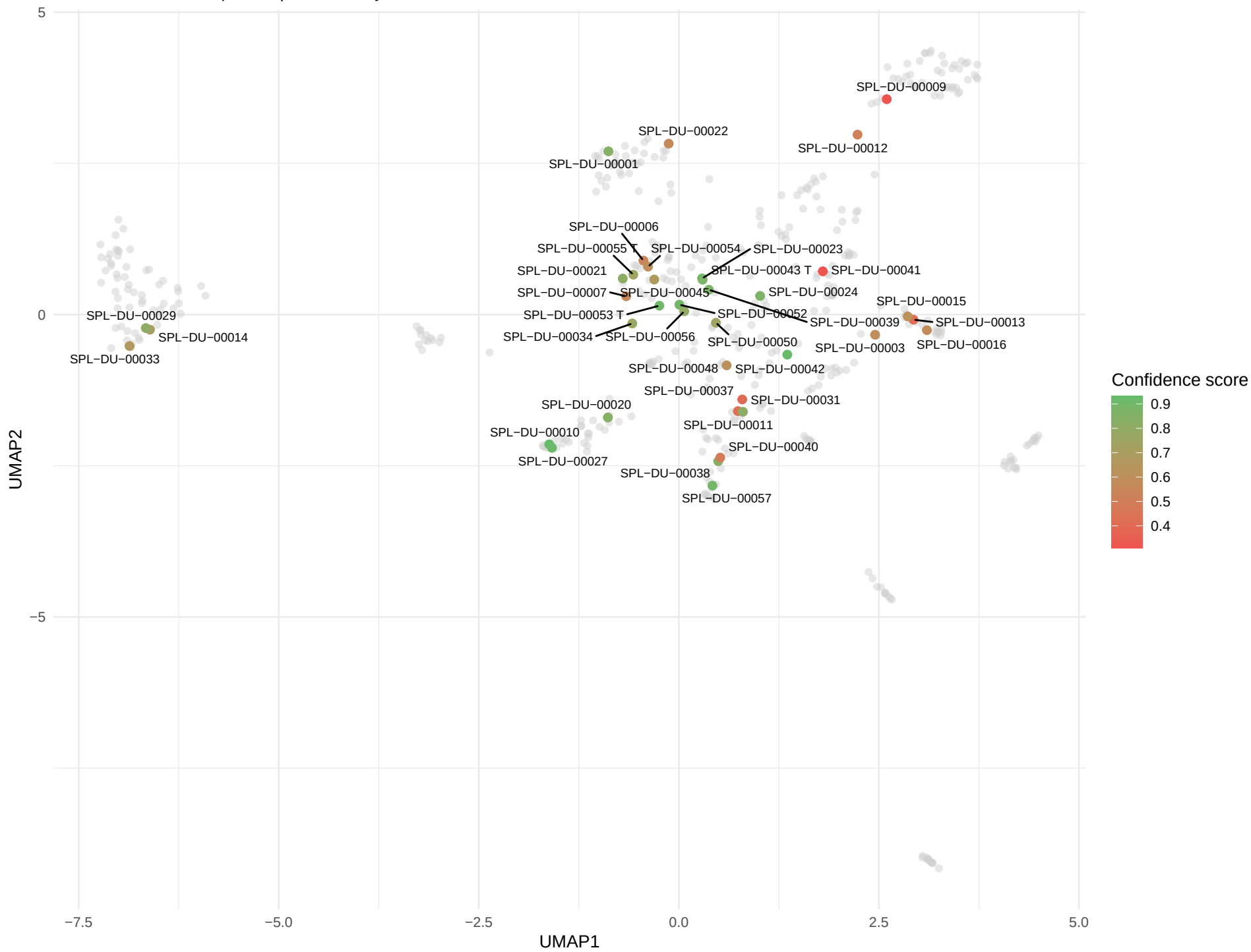
UMAP – RCSI cohort within Jurmeister reference space 20,000 most variable probes | Coloured by classifier confidence score
