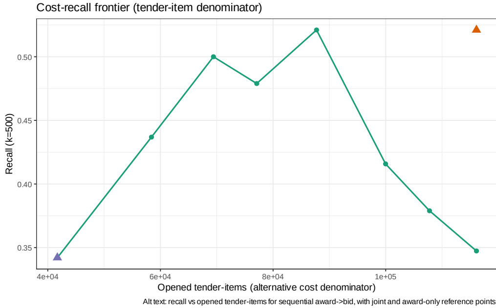
Figure E.1: Recall versus opened tender-items, by ranking rule.
